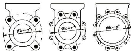
DN 50-65
